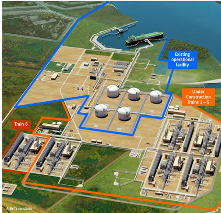
Design production capacity is expected to be ~4.5 mtpa per train, using ConocoPhillips' Optimized Cascade® Process
