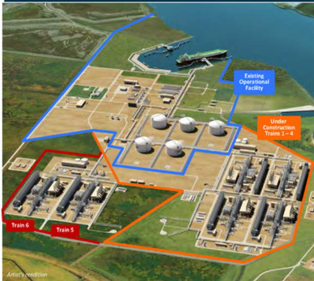
Design production capacity is expected to be ~4.5 MTPA, using ConocoPhillips' Optimized Cascade® Process.
